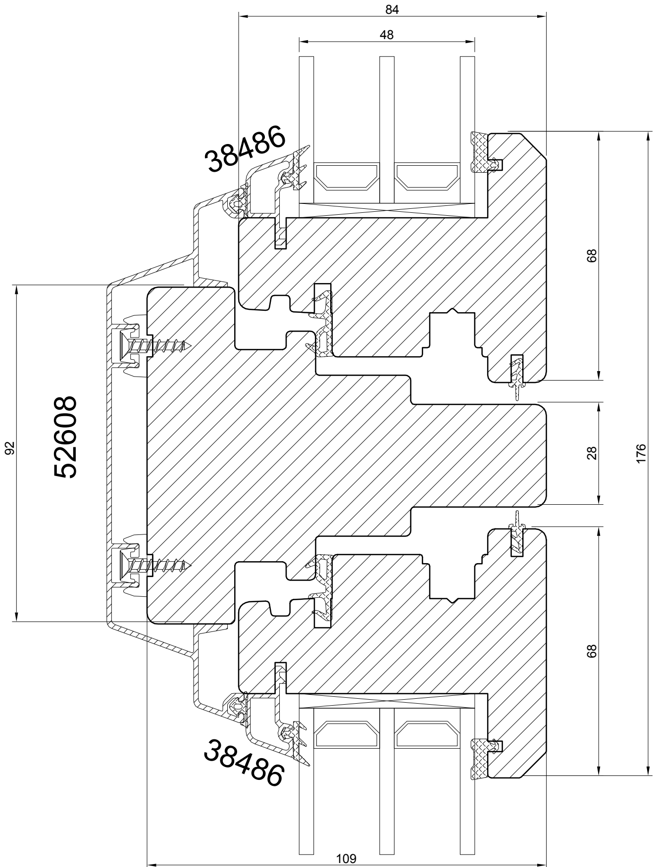
TILT & TURN PASSIVE WINDOW ( inward opening ) with ALU CLAD
